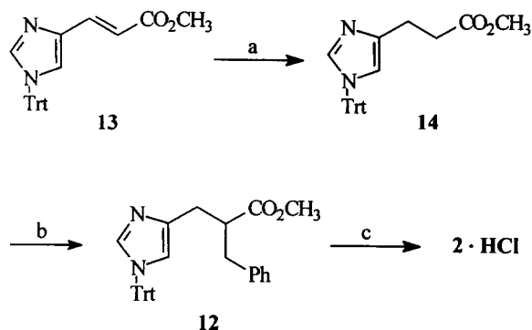
Scheme 3. Reagents, conditions and yields: (a) H 2 , Pd-C, 1 atm, CH 2 Cl 2 -EtOH, 59%; (b) LDA, -78 °C, benzyl bromide, THF, 58%; (c) 10% NaOH, MeOH; 3 N HCl, dioxane, reflux, 65%.
