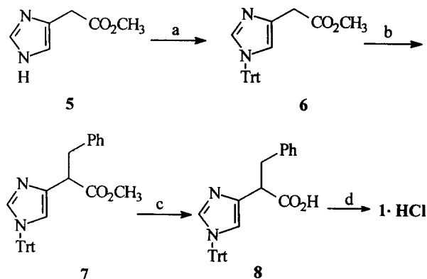
Scheme 1. Reagents, conditions and yields: (a) TrtCl, Et 3 N, DMF, rt, 67%; (b) LDA, -78 °C, benzyl bromide, THF, 61%; (c) 10% NaOH, MeOH, 95%; (d) 3 N HCl, dioxane, reflux, 55%.
