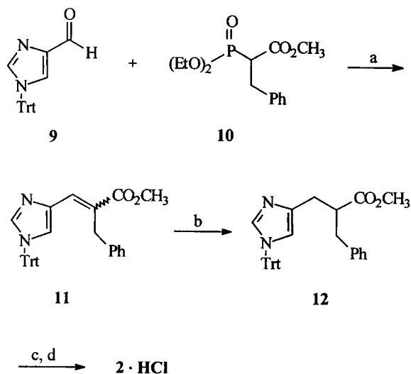
Scheme 2. Reagents, conditions and yields: (a) NaH, THF, 50 °C, 81%; (b) H 2 , Pd-C, MeOH-CH 2 Cl 2 , 1 atm, 92%; (c) 10% NaOH, MeOH, 94%; (d) 3 N HCl, dioxane, reflux, 65%.
